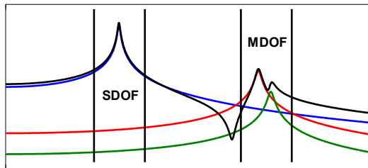
Fig 21 - Curvefitting Different Bands using Different Methods
