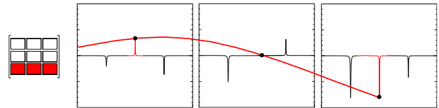
Fig 8c – Mode 2 from Third Row of FRF Matrix
