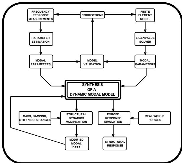
Fig 30 – Overall Dynamic Modeling Process
