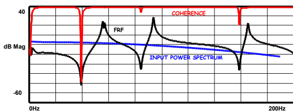
Fig 12b - Hammer Tip Adequate to Excite All Modes
