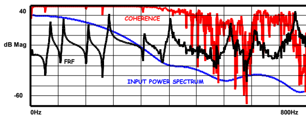
Fig 12a - Hammer Tip Not Sufficient to Excite All Modes
